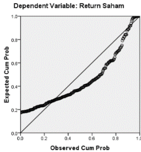
Gambar 1. Scatterplot
