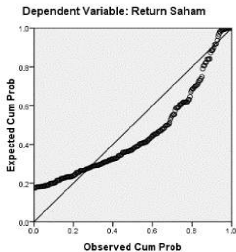
Gambar 1. Scatterplot
